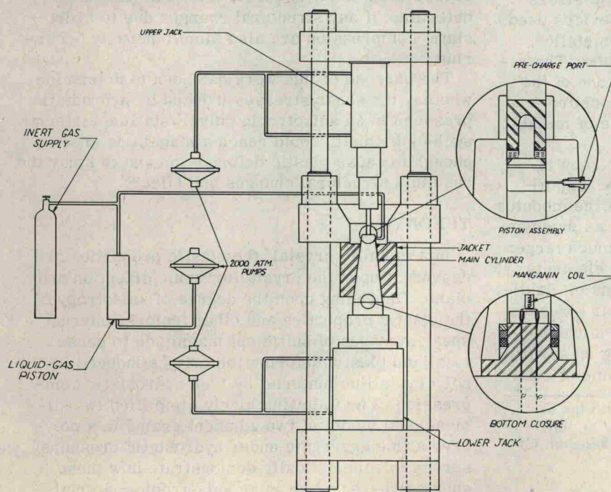
Fig. 1—Schematic of 30,000 atm pressure system.
